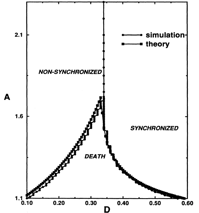
FIG. 1. Phase diagram for a pair of coupled oscillators with frequencies \pi/6 and \pi/2 . A is a parameter that measures the attraction to limit cycle and D is the coupling strength. The nonsynchronized and synchronized regions correspond to parameter values such that the oscillators have different and equal asymptotic frequencies, respectively. In the region labeled as death, the rest state is stable. The boundary of this region can be calculated by a linear stability analysis.
