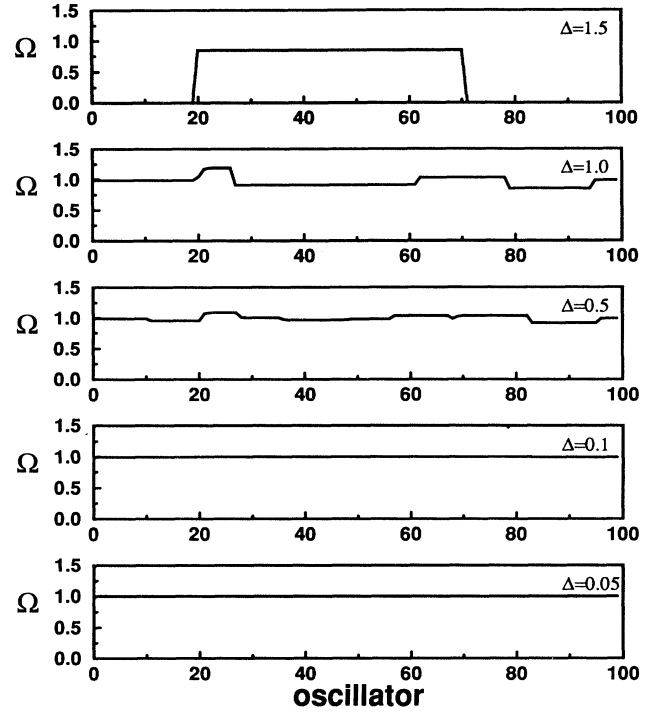
FIG. 5. The asymptotic frequency \Omega of a chain after 3000 time steps for frequency distributions of different widths, D=0.8 and A=1.1 . Dead oscillators are represented by \Omega=0 .
